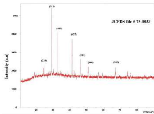
Fig 9: Xrd Spectrum of Encapsulated Fe 3 O 4 Nanoparticles
