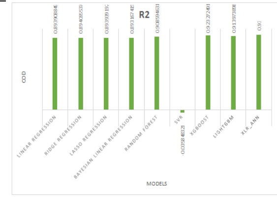
Figure 4: R² Comparison Across Models
