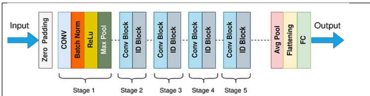
Figure 1. ResNet- 50 structure
