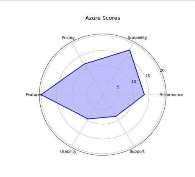
Figure.4: Azure Scores
