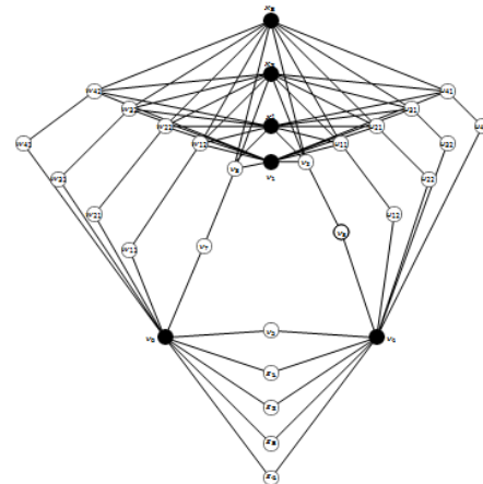
Figure 8: A graph G with \text{rad. } G = \text{diam. } G = 4 and s_{it}(G) = 6
