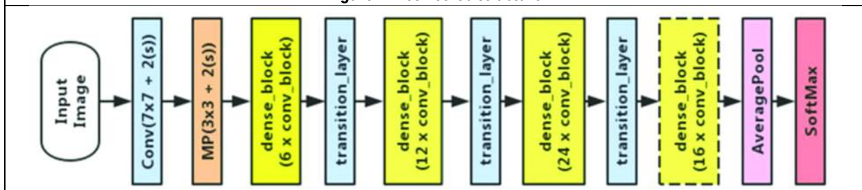
Figure 2 DenseNet121 structure
