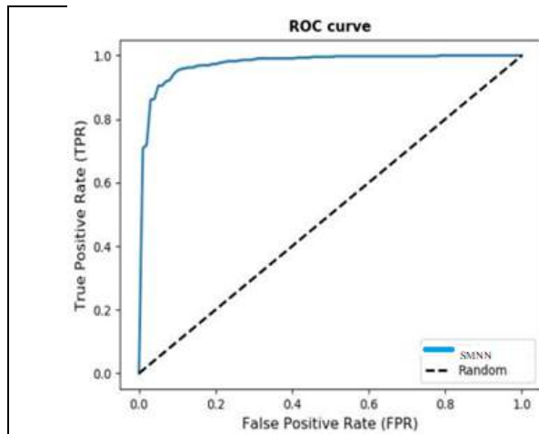
Figure 9 : ROC curve
