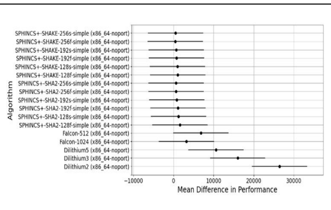
Figure. 2: Comparison of Top-Performing Algorithm
