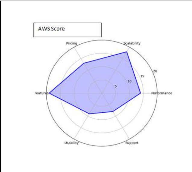
Figure.3: AWS Score
