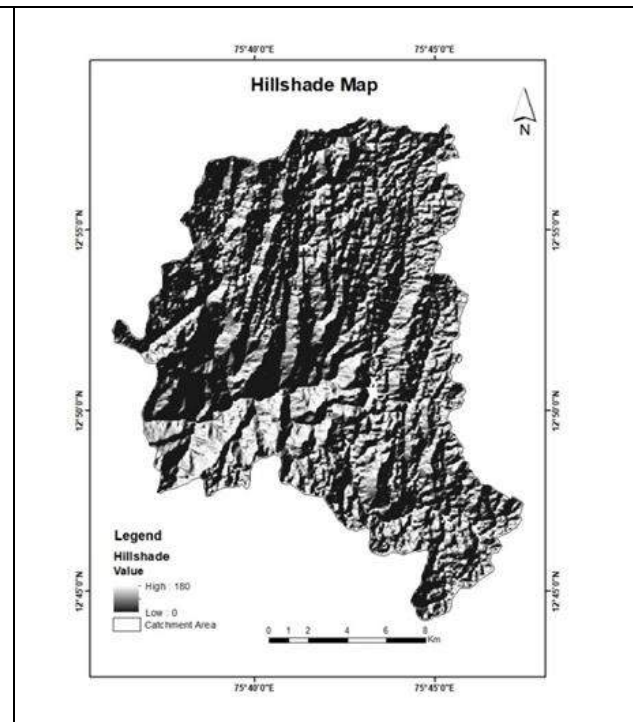
Figure.6: Representing the hillshade map of the Yethinahole catchment area.
