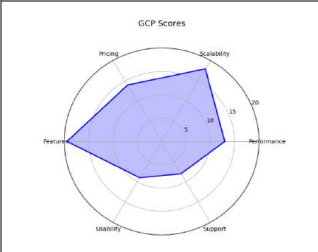
Figure.5:GCP Scores
