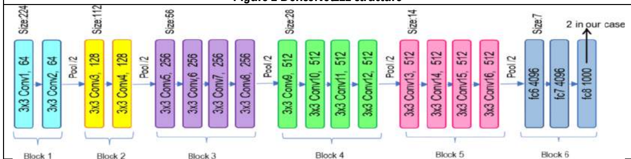
Figure 3 VGG19 Structure
