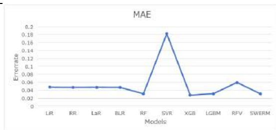
Figure 8.Comparative results of MAE
