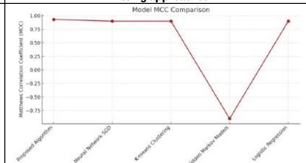
Figure 4: Model MCC Comparison with Proposed and Existing approaches
