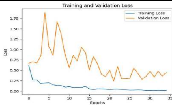
Figure.9: Training and validation Loss
