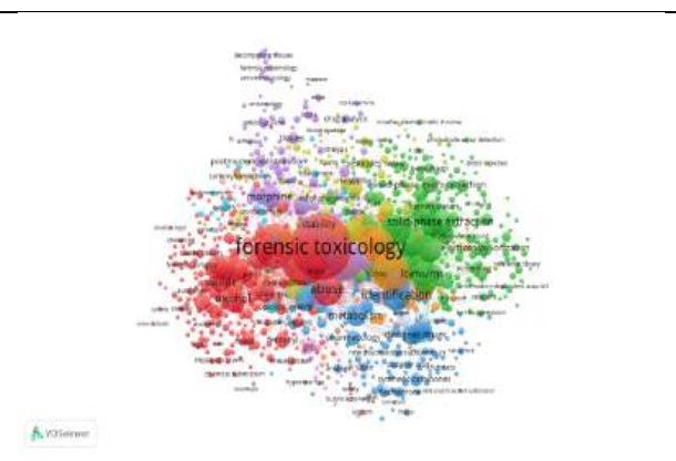
Figure 2 : Keyword Frequency
