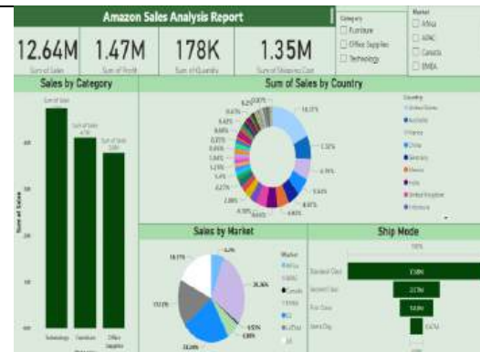
Figure 4: Overview Dashboard
