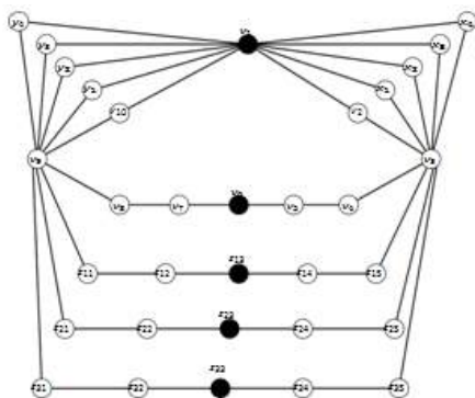
Figure 7: A graph G with \text{rad. } G = \text{diam. } G = 3 and s_{it}(G) = 6
