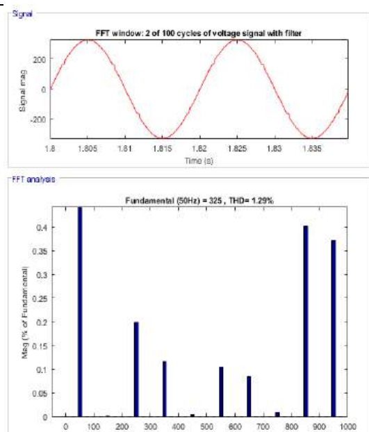
Figure 6 Matlab FFT Analysis of Voltage with Filter
