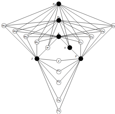
Figure 7: A graph G with \text{rad. } G = \text{diam. } G = 3 and s_{it}(G) = 6
