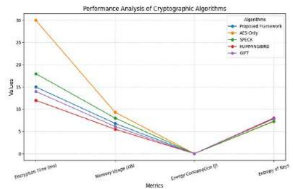
Figure 2: Performance Analysis
