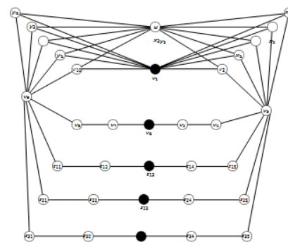
Figure 10: A graph G with \text{rad. } G = \text{diam. } G = 5 and s_{it}(G) = 6
