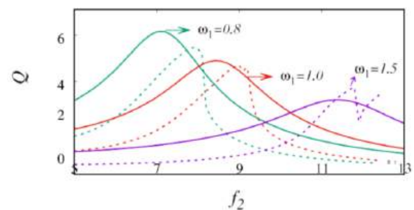
Fig. 4 Relationship between f_2 and the response amplitude Q . The solid line represents analytically computed response amplitude and the dotted line represents the numerical response amplitude for different values of \omega_1 and that curves for \omega_1 0.8, 1.0 and 1.5 are represented by different colors.
