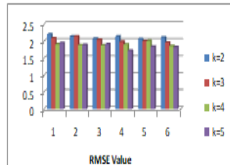
Fig.2.RMSE value for different latent factors of SMRR dataset
