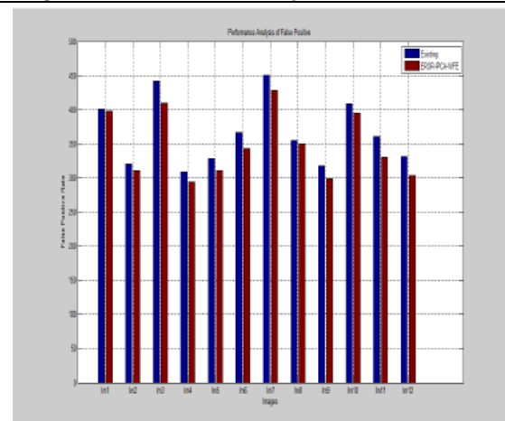
Figure .4 Performance Analysis of False Positive
