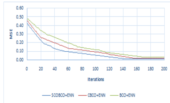
Figure 8: Convergence analysis for the CIC-DDoS2019 dataset
