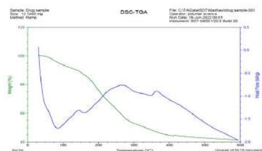
Figure.4.b. DSC thermogram of irbesartan loaded microbeads
