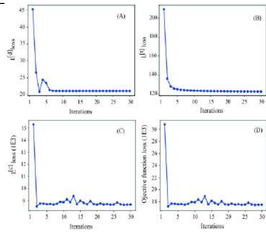
Figure 10: Convergence examination of SMNN using several strategies: objective function loss versus iteration count for A L[d] loss, B L[t] loss, C L[c] loss, and D
