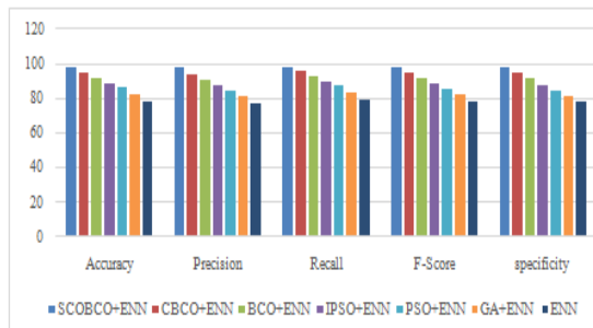
Figure 3 : Performance results for the CIC-IDS2017 dataset
