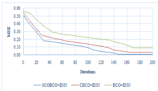
Figure 5: Convergence analysis for the NSL-KDD dataset
