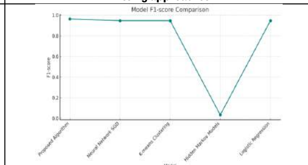
Figure 6: Model F1-Score Comparison with Proposed and Existing approaches
