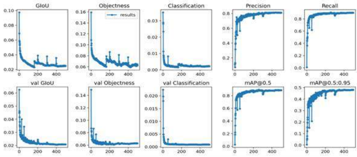
Figure. 3: Simulation results obtained on Scaled-YOLOv4 for Field Hockey Dataset (Epochs: 500)
