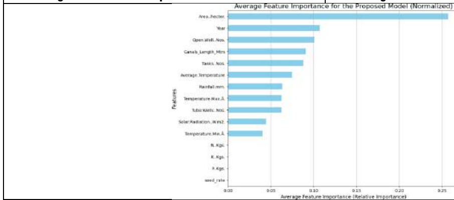
Figure 6: Average Feature Importance of the Proposed XLR_ANN Model
