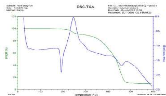
Figure.4.a: DSC thermogram of pure drug (Irbesartan)
