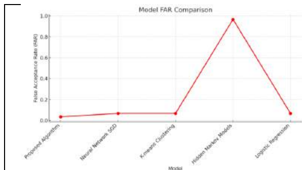
Figure 1: Model FAR Comparison with Proposed and Existing approaches
